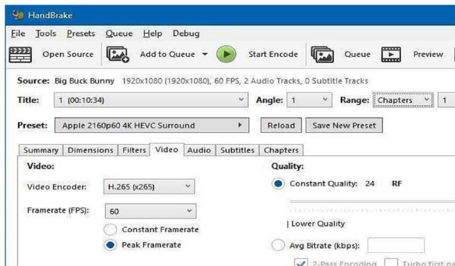
Figure 9. HandBrake software
