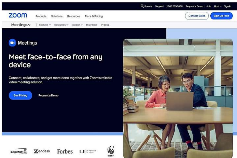
Figure 12. Zoom client
